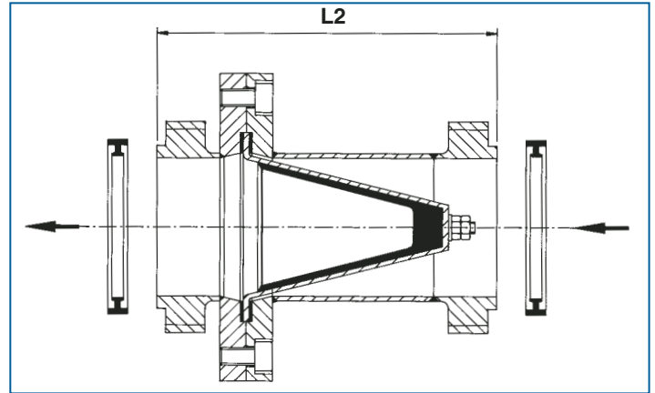
IDF Connections
